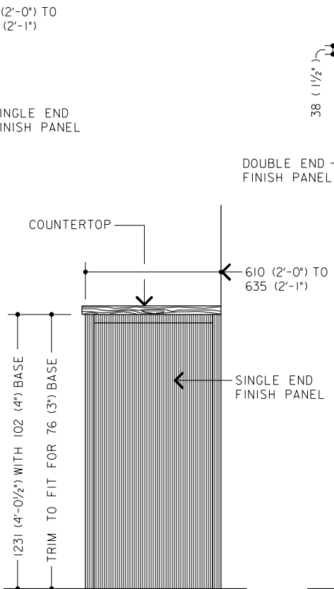
ELEVATION D ( ALTERNATE )
