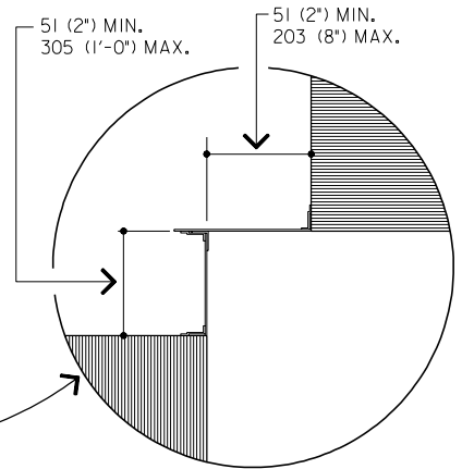
DETAIL "A" INSIDE CORNER
