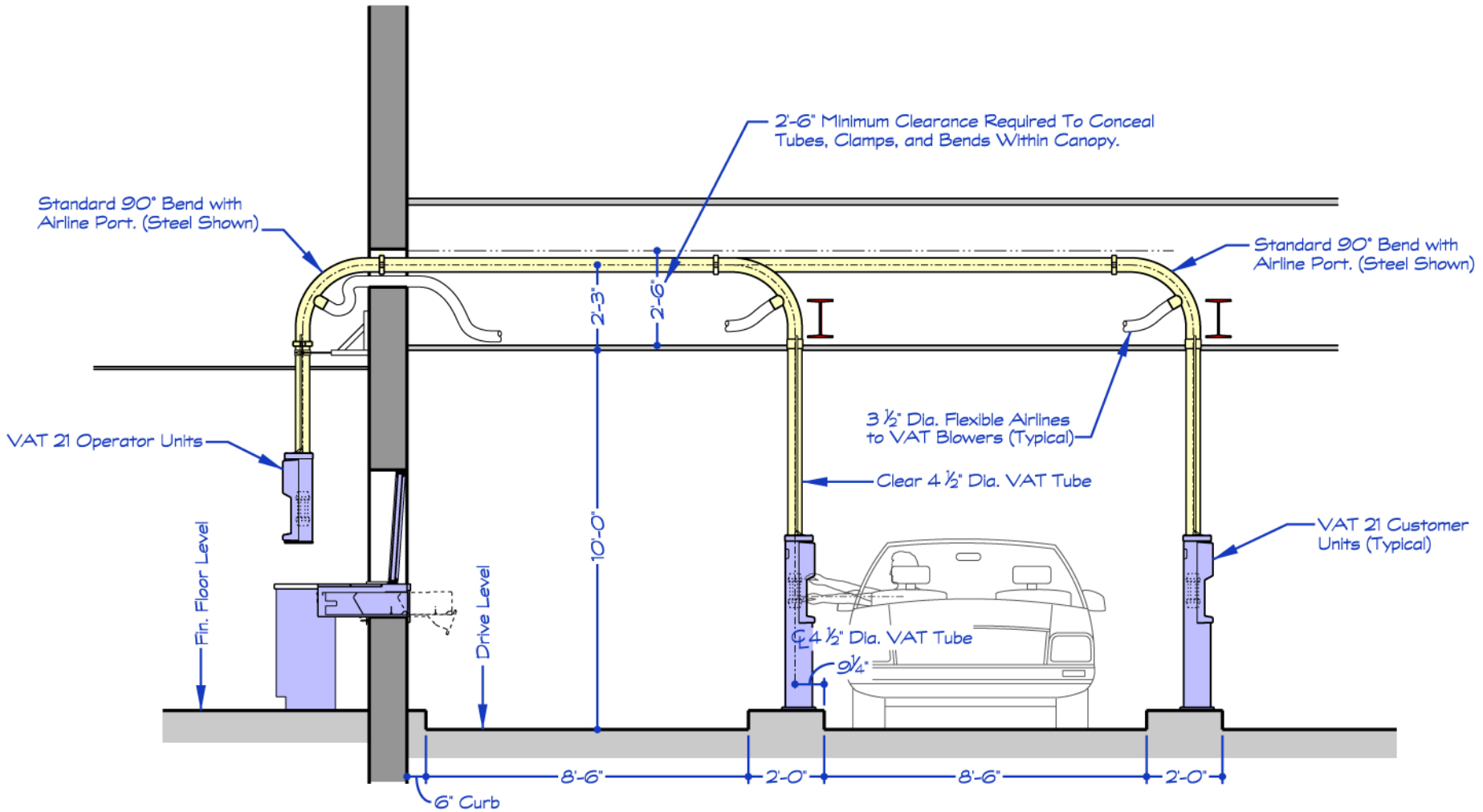
Section (Typical Tube Run with No Interference)
